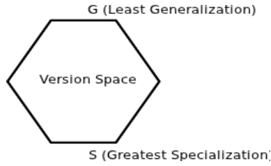
Figure 1: Version Space
